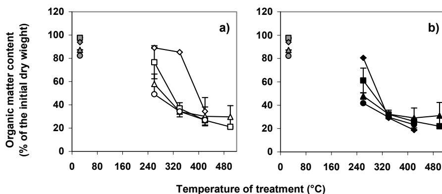
Figure 2: Residual organic matter, as percentage of the initial dry weight, after thermal treatment at 260, 340, 420 and 500 °C for 20 min (a, open symbols) or 40 min (b, solid symbols). Symbol meaning: squares, WO (U=9%); triangles, PM_I (U=10%); circles, PM_II (U=14%); diamonds, PM_III (U=71%). The grey symbols indicate the organic matter content of the untreated material. Bars are the SD of the mean, when available.
