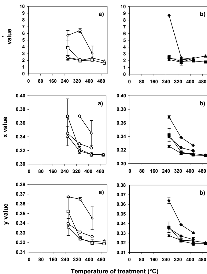
Figure 3: Values of the chromaticity coordinates, Y, x and y, after thermal treatment at 260, 340, 420 and 500 °C for 20 min (a, open symbols) or 40 min (b, solid symbols). Symbol meaning: squares, WO (U=9%); triangles, PM_I (U=10%); circles, PM_II (U=14%); diamonds, PM_III (U=71%). Bars are the SD of the mean, when available.
